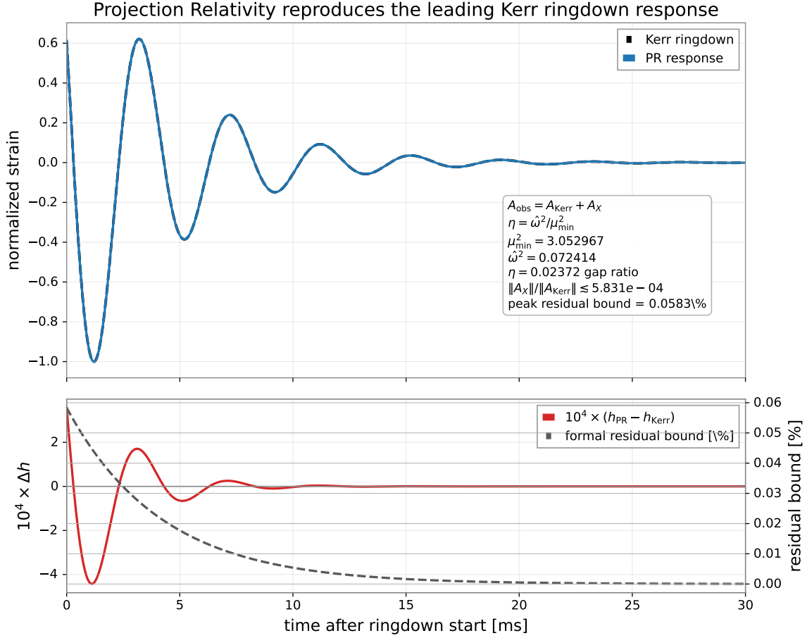
Figure 8: Kerr-consistent gravitational-wave response. In the exterior low-energy regime, Projection Relativity recovers the Kerr ringdown hierarchy rather than replacing it. The observable response decomposes as A_{\text{obs}} = A_{\text{Kerr}} + A_X , with the projection-sector residual A_X suppressed by the radial spectral gap. For the illustrative mode shown here, \eta = \hat{\omega}^2/\mu_{\text{min}}^2 = 0.0237 , while the Newton-normalized residual bound gives \|A_X\|/\|A_{\text{Kerr}}\| \lesssim 5.83 \times 10^{-4} . The top panel shows the resulting Kerr/PR waveform overlap; the bottom panel magnifies the residual correction.
