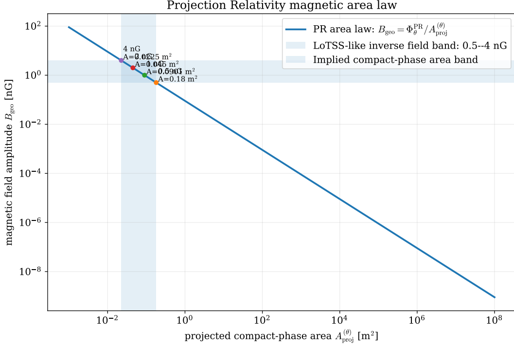
Figure 6: Projection Relativity magnetic area law. The compact phase sector fixes the flux normalization \Phi_\theta^{\text{PR}} = (\hbar/e)(Z_A/c_{\text{bc}}) , while the realized magnetic domain supplies the projected compact-phase area A_{\text{proj}}^{(\theta)} . The resulting field is B_{\text{geo}}^{\text{PR}}[\text{nG}] = 0.09009597185/A_{\text{proj}}^{(\theta)}[\text{m}^2] . The shaded band shows the compact-phase areas corresponding to the foreground-cleaned LoTSS-scale residual field range.
