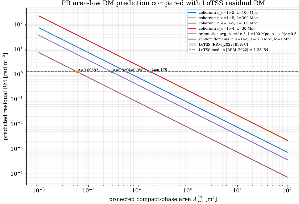
Figure 7: PR area-law RM prediction compared with LoTSS residual RM. For each plasma/window model, the PR area law predicts a residual Faraday rotation through \text{RM}_{\text{pred}} = 812 n_e L W_{\text{EM}} (0.09009597185 / A_{\text{proj}}^{(\theta)}) . The horizontal band shows the foreground-cleaned LoTSS residual |\text{RRM}_{2022}| = 1.254538 \text{ rad m}^{-2} with its bootstrap confidence interval. Intersections determine the projected compact-phase area required by each physical window model.
