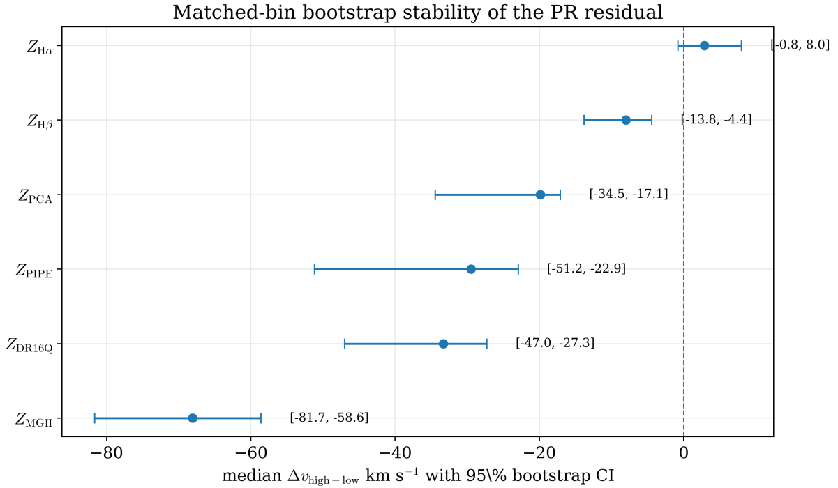
Figure 5: Matched-bin bootstrap stability of the PR residual. Stability analysis of the PR-predicted velocity residual using matched-bin bootstrap resampling. The primary redshift estimators show negative locked 95% confidence intervals, confirming that the observed residual is a statistically robust feature rather than a random-bin artifact.
